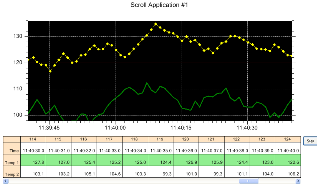
A RTProcessVarViewer displaying two RTProcessVar objects
